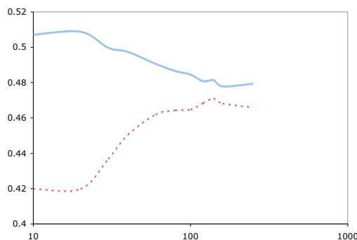
Figure 1: Relation between context length and correlation to income per screen: positive references, pre-release (blue, continuous line) and non-neutral references, post-release (red, dashed line)
